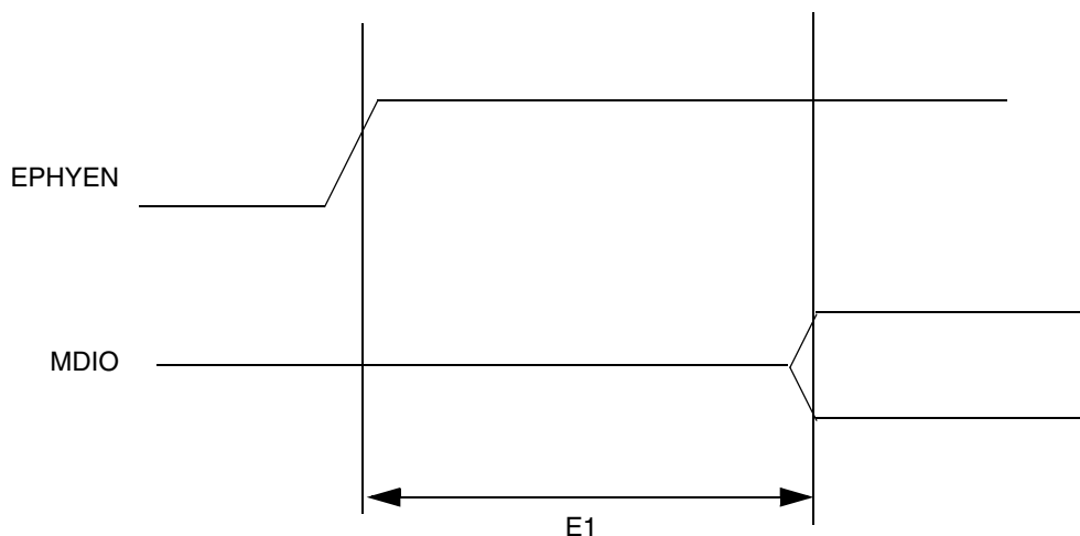
Figure 9. EPHY Timing
