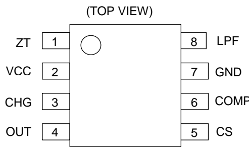
Figure 2. Pin Configuration
