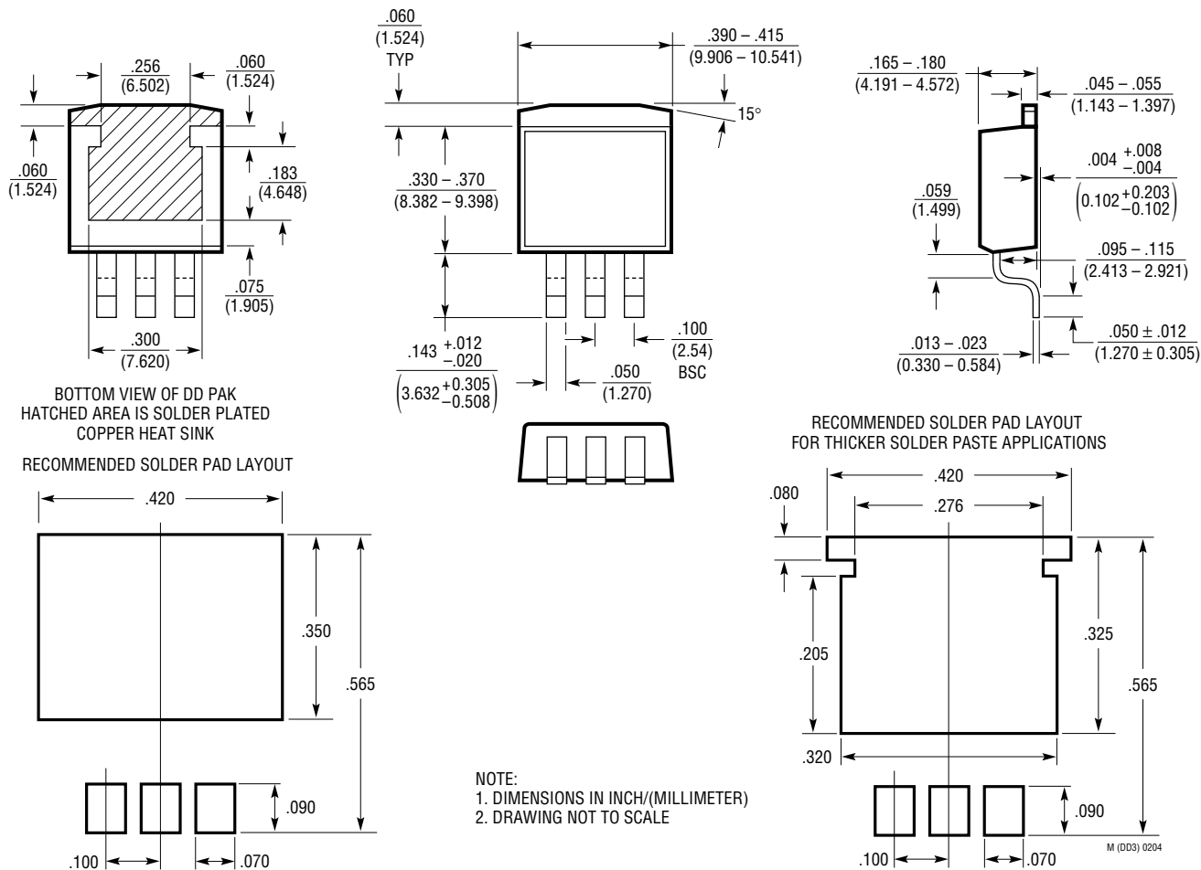
M Package 3-Lead Plastic DD Pak (LTC DWG # 05-08-1460)
