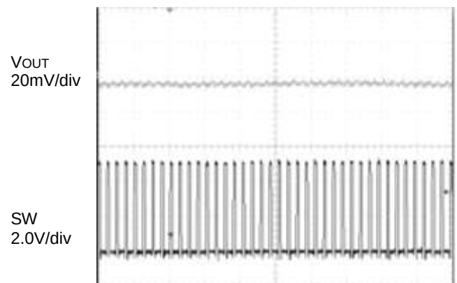
Figure 42. Switching Waveform at PWM Control ( V_{IN}=5.0V , V_{OUT}=1.2V , I_{OUT}=4A )
