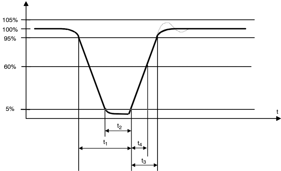
Figure 2. 100% Modulation Waveform
