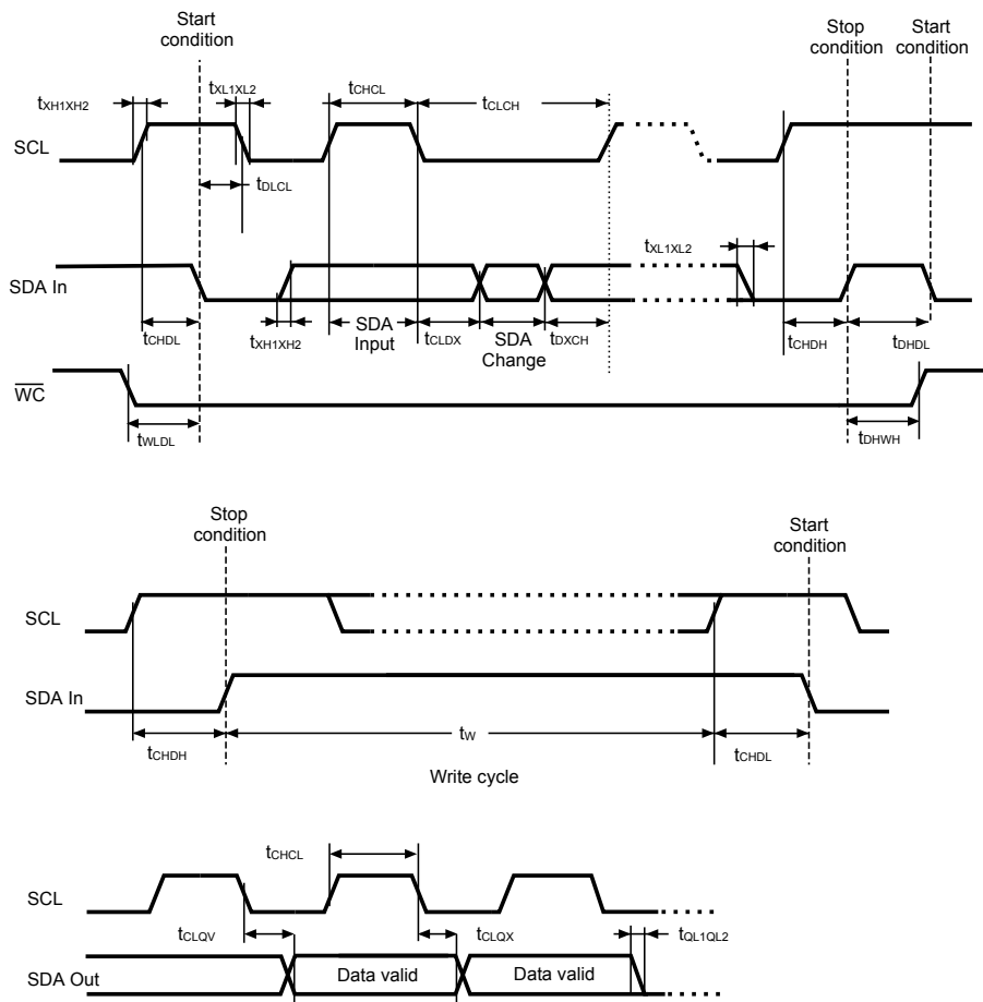
Figure 12. AC waveforms
