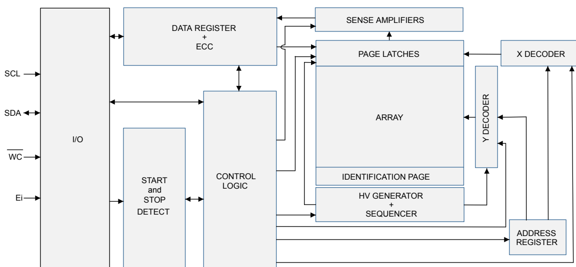
Figure 1. Logic diagram
