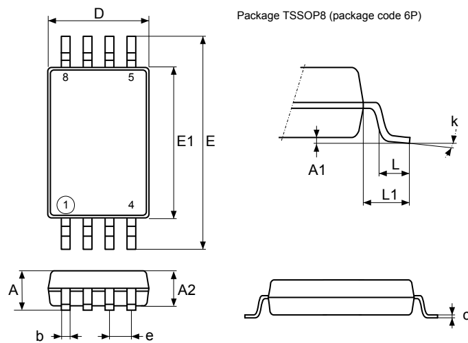
Figure 13. TSSOP8 – Outline
