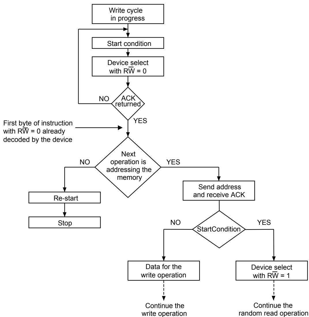
Figure 7. Write cycle polling flowchart using ACK
