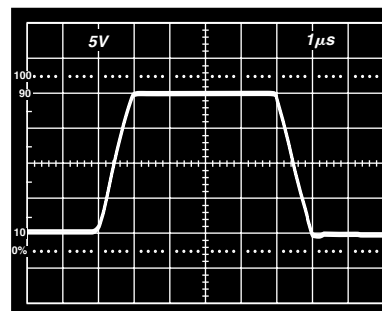
Figure 14. Transient Response R_L = 2\ \text{k}\Omega , C_L = 500\ \text{pF}
