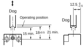
One-way Roller Arm Lever (Horizontal) (D4N-□□62)
