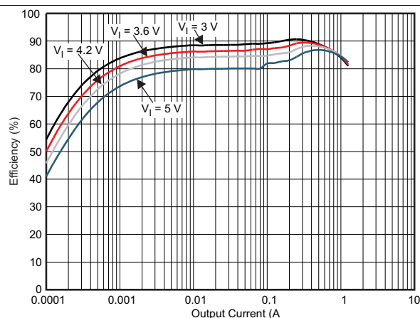
DCDC2 V_O = 1.8 V LQM2NPN-1 \mu H PFM Mode 25°C
