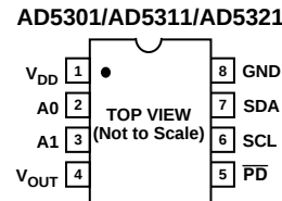
8-Lead \mu SOIC (RM-8)
