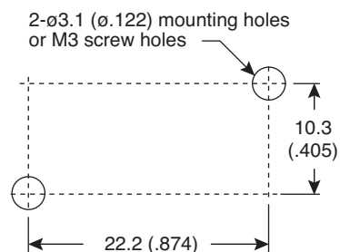
Mounting Holes
