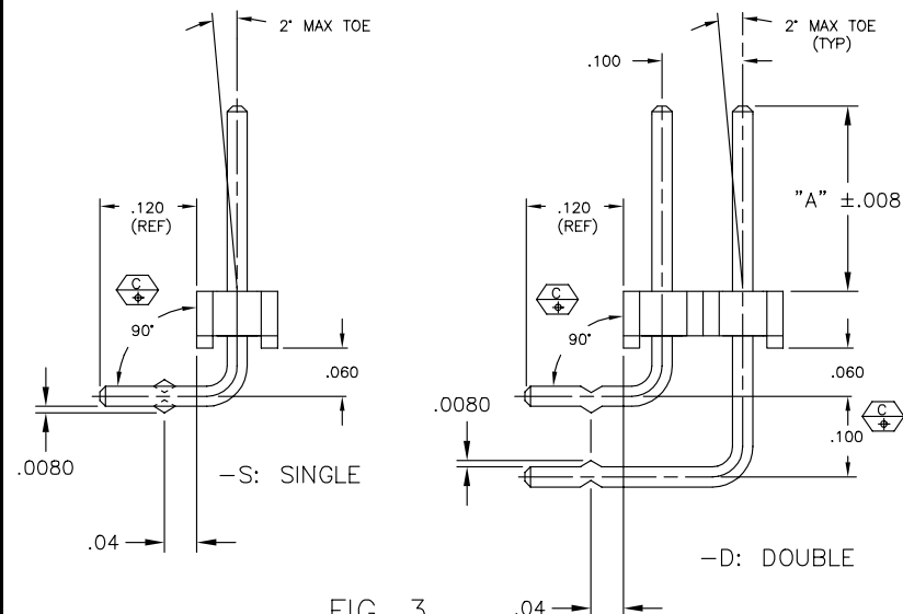
FIG. 3 (-LA OPTION) NOTE: END VIEWS SHOWN.
