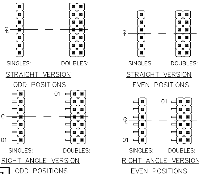
FIG. 2 (-RA OPTION) NOTE: END VIEWS SHOWN.
