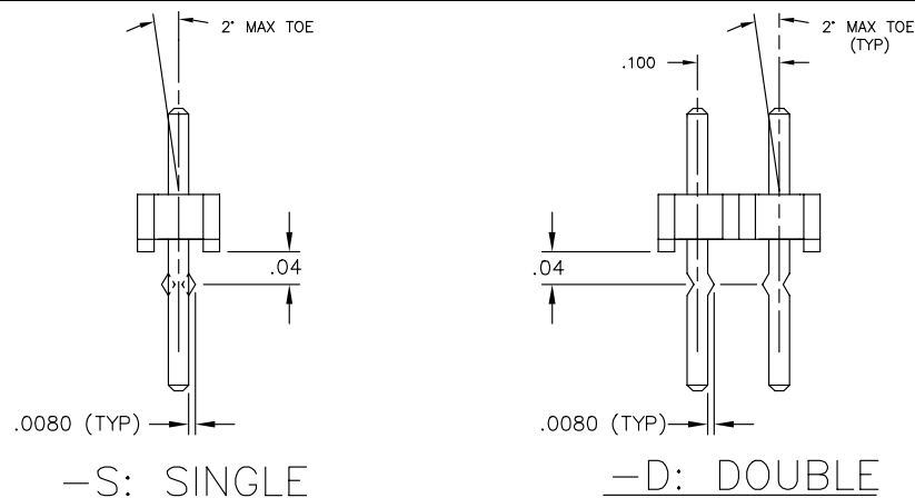
FIG. 3 (-LA OPTION) NOTE: END VIEWS SHOWN.
