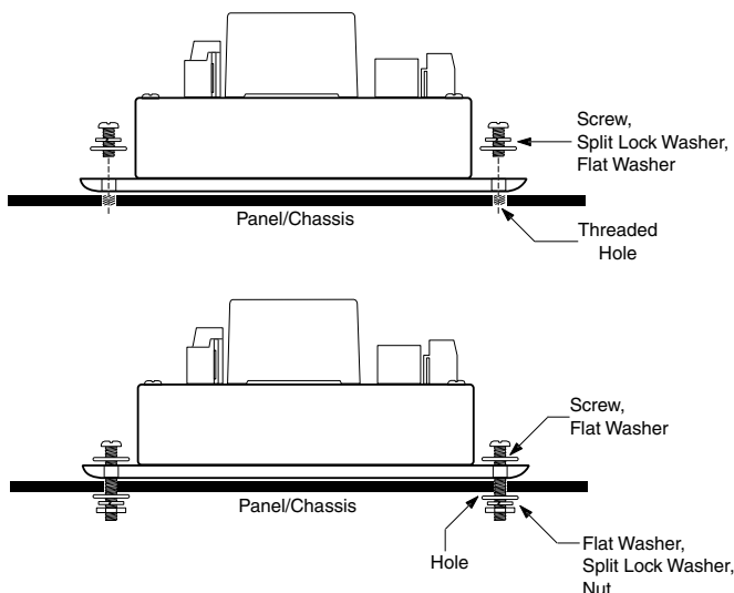
Figure 4. Chassis Mounting
