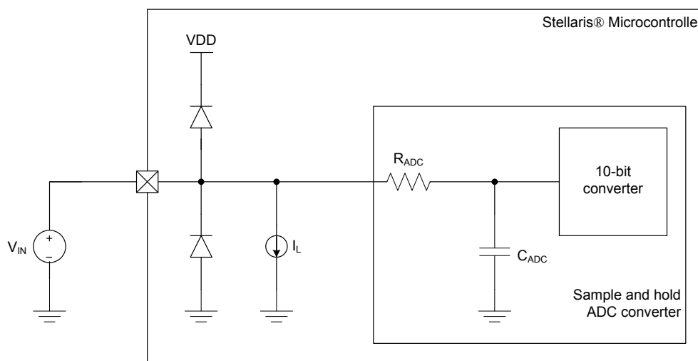
Figure 20-10. ADC Input Equivalency Diagram
