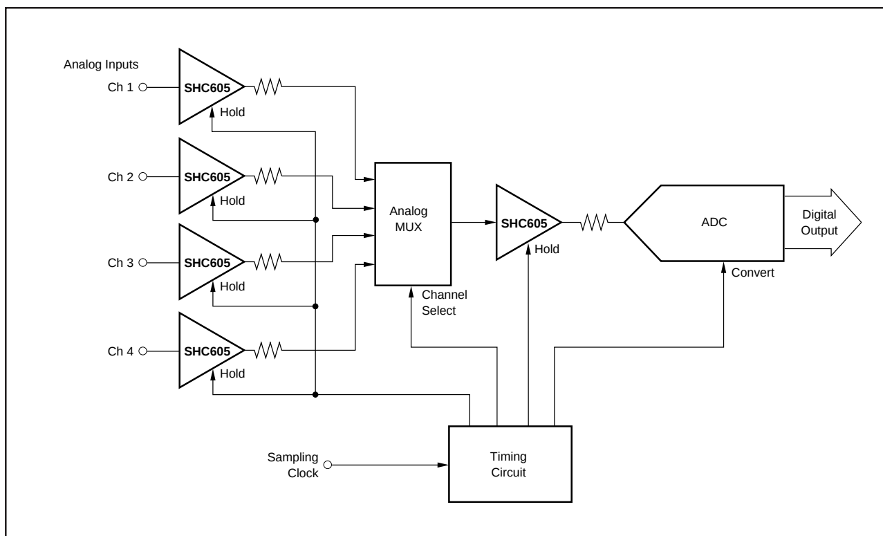
FIGURE 13. Multi-Channel Simultaneous Sampling System.
