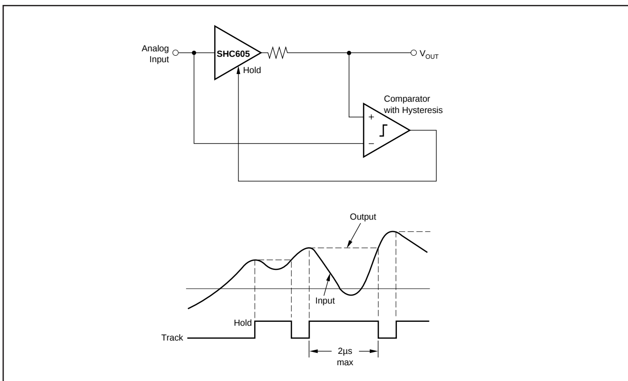
FIGURE 15. High-Speed Peak Detector.
