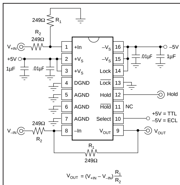
FIGURE 6. Differential Gain of 1 Track-and-Hold Amplifier.
