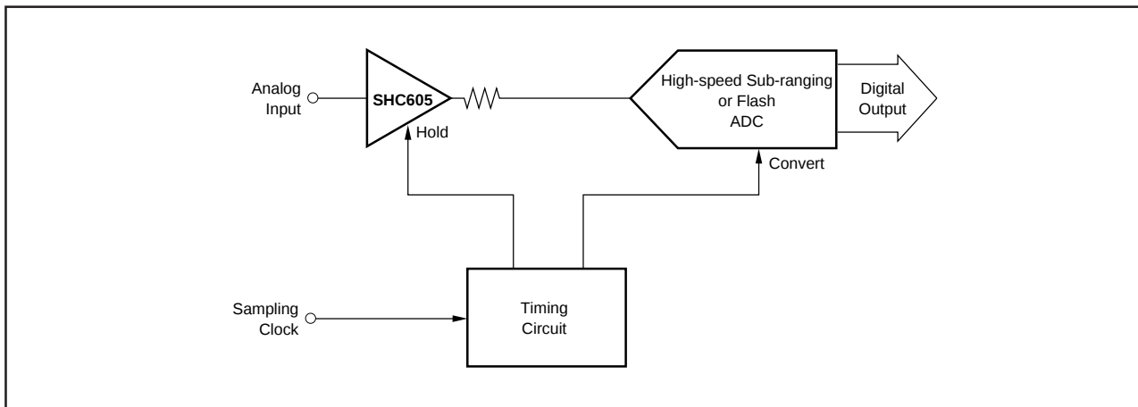
FIGURE 11. Sampling ADC.
