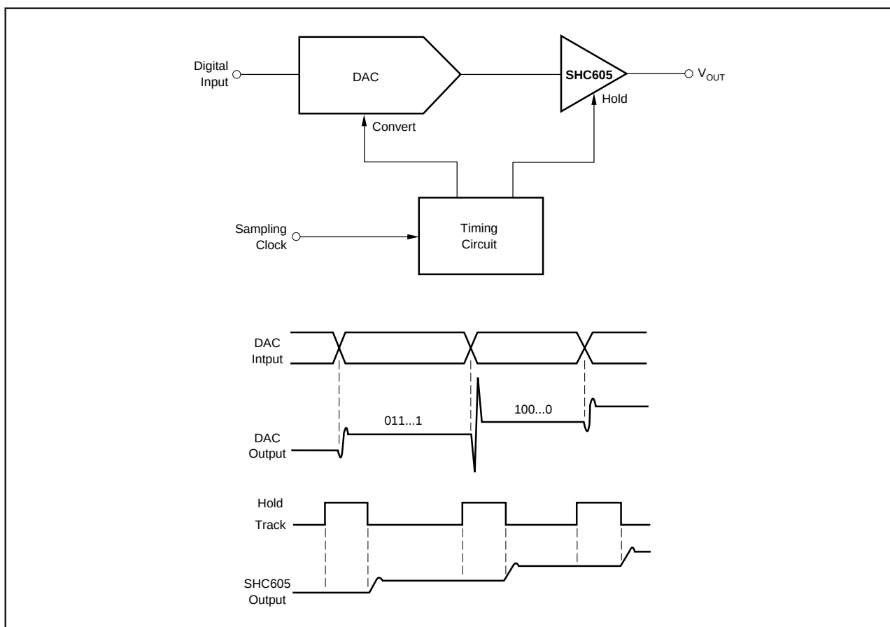
FIGURE 16. DAC Deglitcher.
