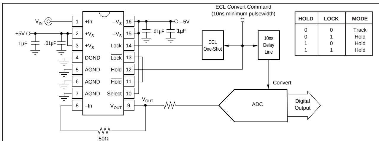
FIGURE 7. Edge-Triggered ADC.
