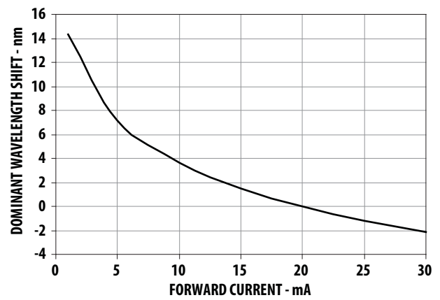
Figure 4. Relative Dominant Wavelength vs Forward Current
