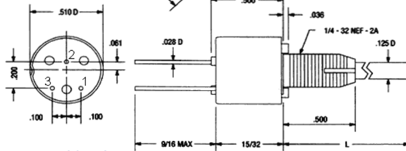
LOCKING BUSHING
