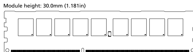
Figure 2: 240-Pin UDIMM (MO-269 R/C E3)
