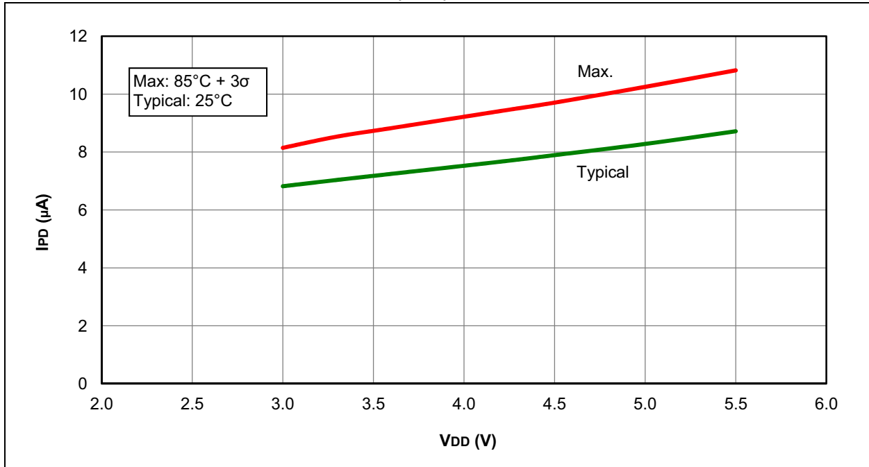
FIGURE 30-39: I_{PD} , BROWN-OUT RESET (BOR), BORV = 0, PIC16F1508/9 ONLY
