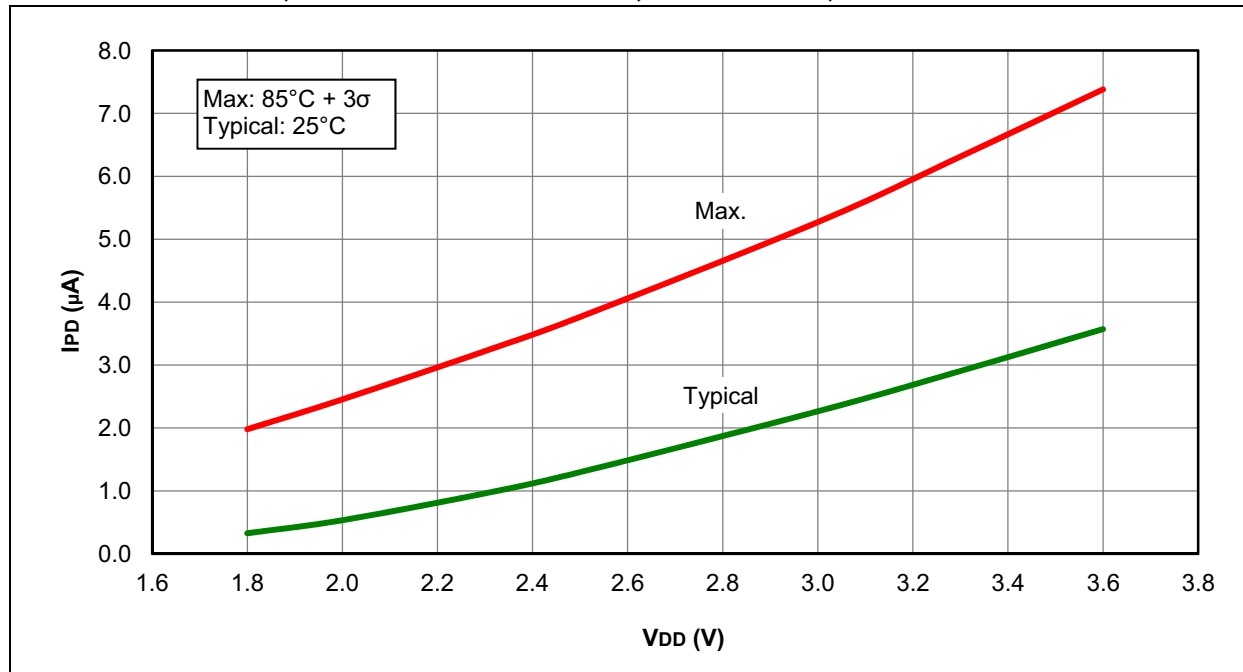
FIGURE 30-41: I_{PD} , SECONDARY OSCILLATOR, F_{osc} = 32\text{ kHz} , PIC16LF1508/9 ONLY
