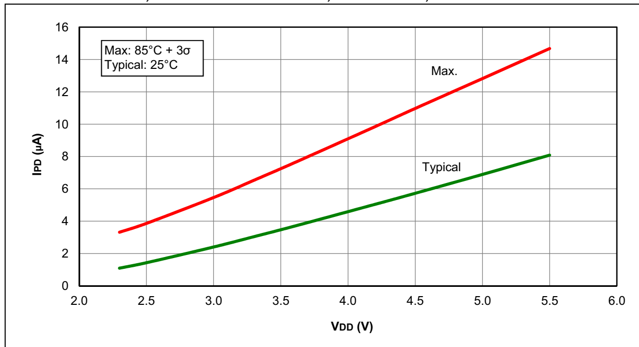
FIGURE 30-42: I_{PD} , SECONDARY OSCILLATOR, F_{osc} = 32\text{ kHz} , PIC16F1508/9 ONLY
