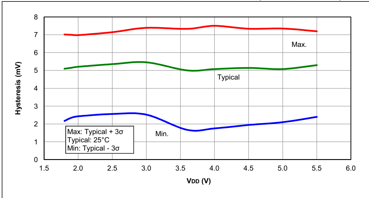
FIGURE 30-66: COMPARATOR HYSTERESIS, LOW-POWER MODE ( CxSP = 0 , CxHYS = 1 )
