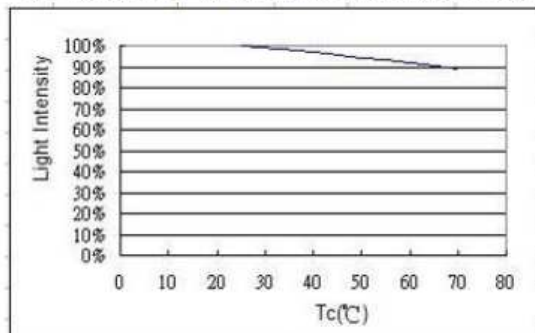
Temperature vs Relative Luminous Flux
