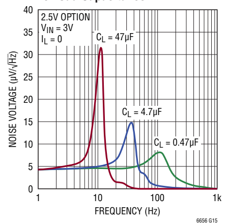
Output Noise Voltage Spectrum vs Load Capacitance
