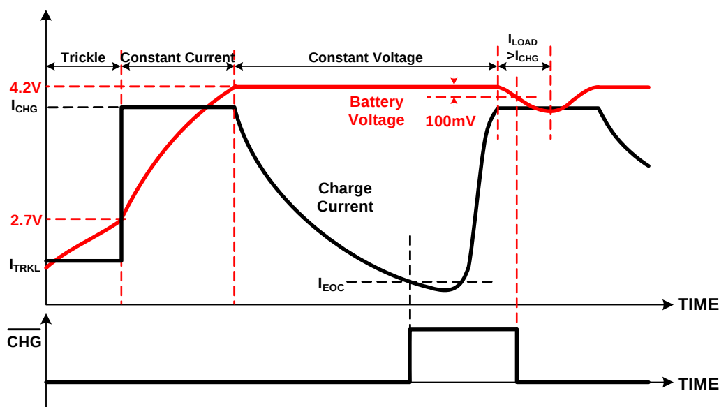
Figure 27. Charge Profile
