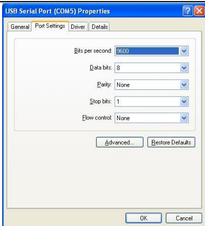
Figure 2.9 - Settings Tab
