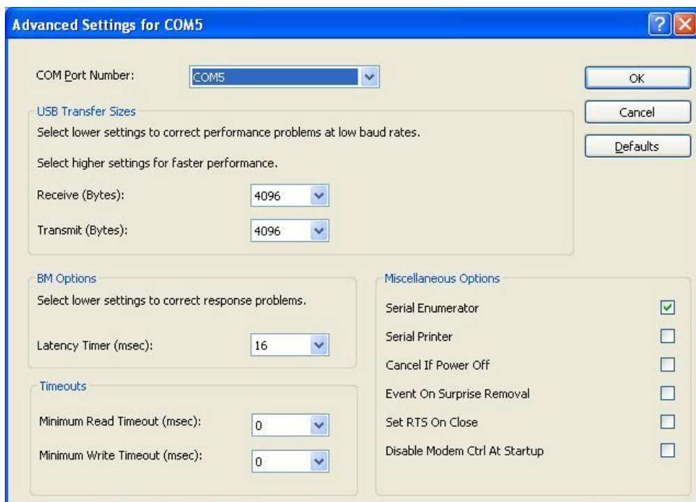
Figure 2.10 - Advanced Options
