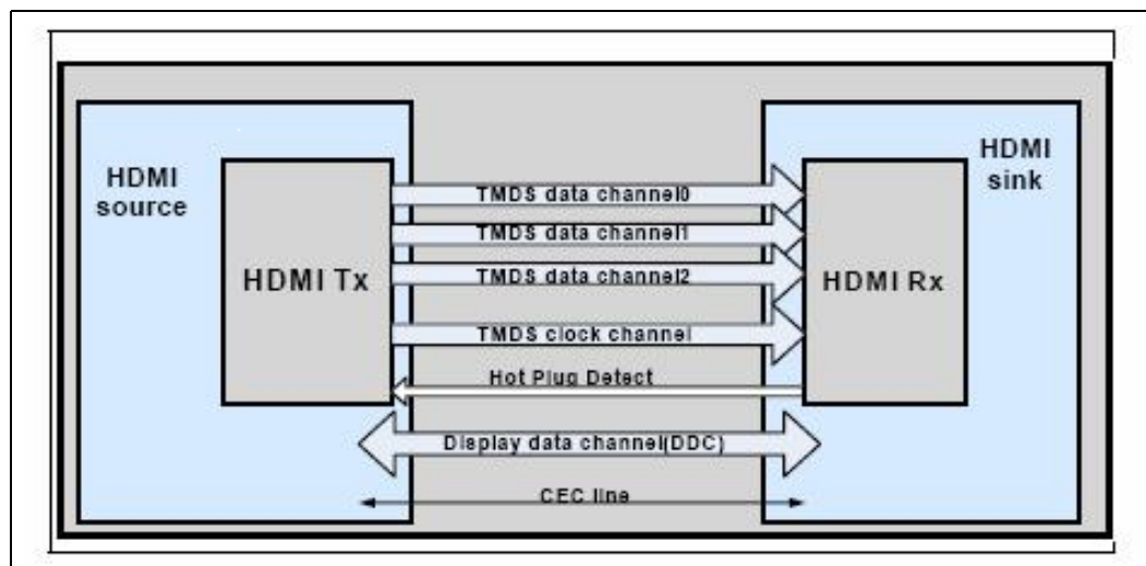
Figure 5-17. HDMI Overview
