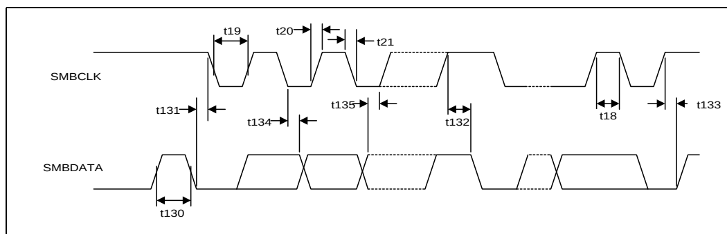
Figure 8-21. SMBus Timeout
