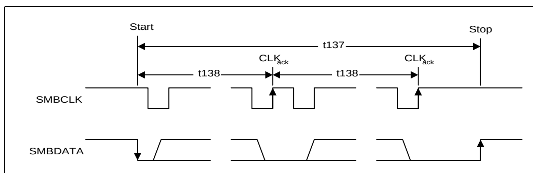
Figure 8-21. SMBus Timeout
