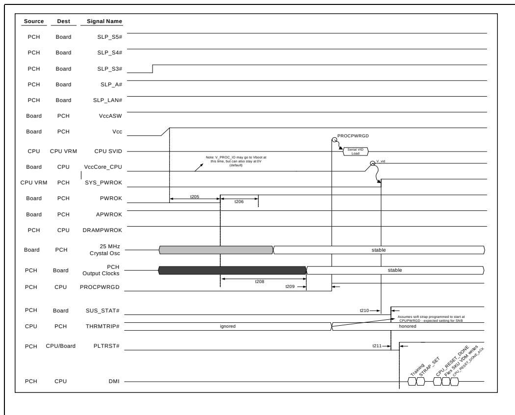
Figure 8-5. S5/Moff - S5/M3 Timing Diagram
