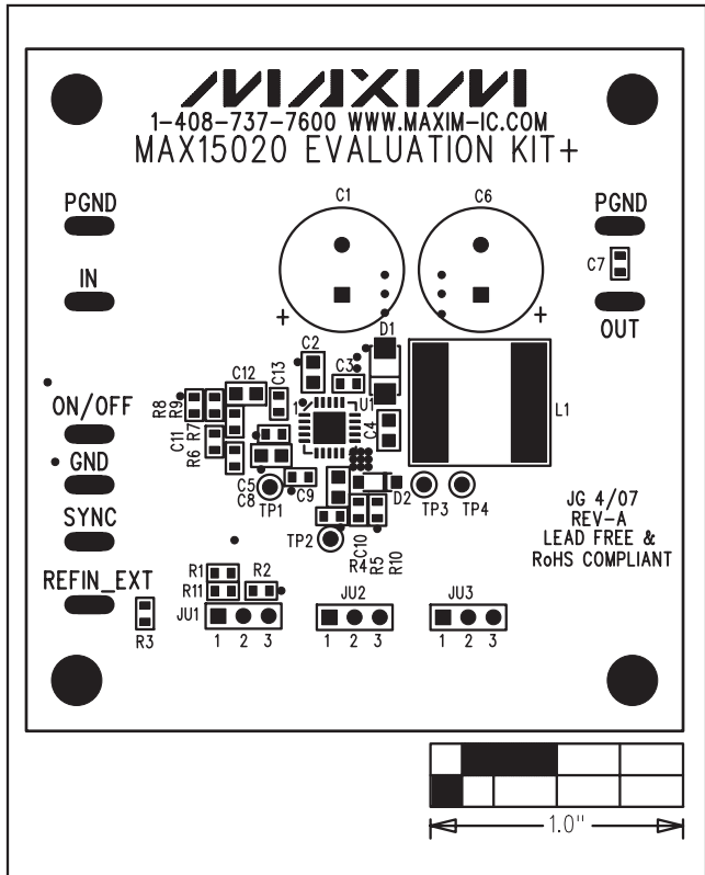
Figure 2. MAX15020 EV Kit Component Placement Guide—Component Side
