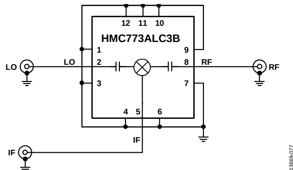
Figure 77. Typical Application Circuit
