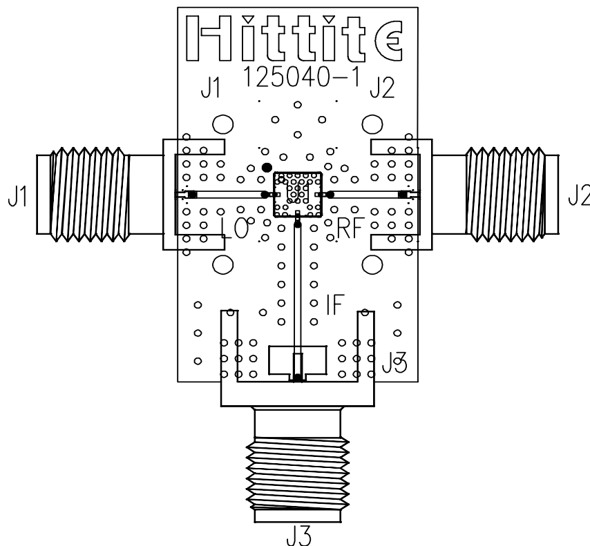
Figure 78. Evaluation PCB
