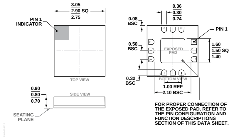
Figure 79. 12-Terminal Ceramic Leadless Chip Carrier [LCC] (E-12-4)
