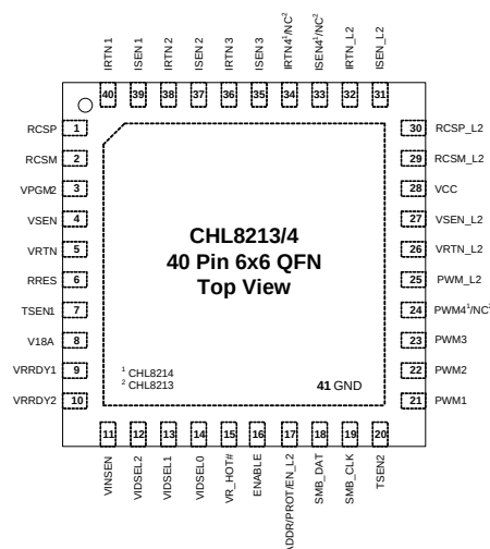
Figure 1: CHL8213/14 Package Top View
