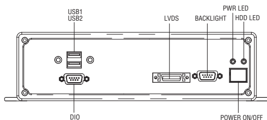
Front Panel External I/O Mechanical Layout/Drawing
