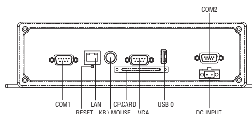
Rear Panel External I/O Layout/Drawing
