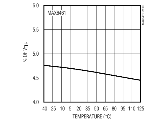
HYSTERESIS vs. TEMPERATURE
