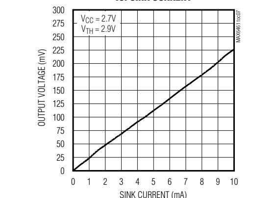
OUTPUT VOLTAGE LOW vs. SINK CURRENT
