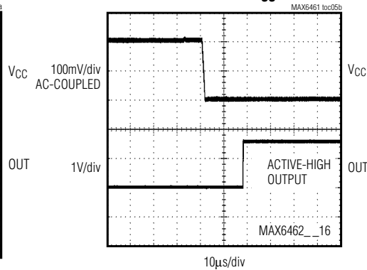
PROPAGATION DELAY V_{CC} FALLING
