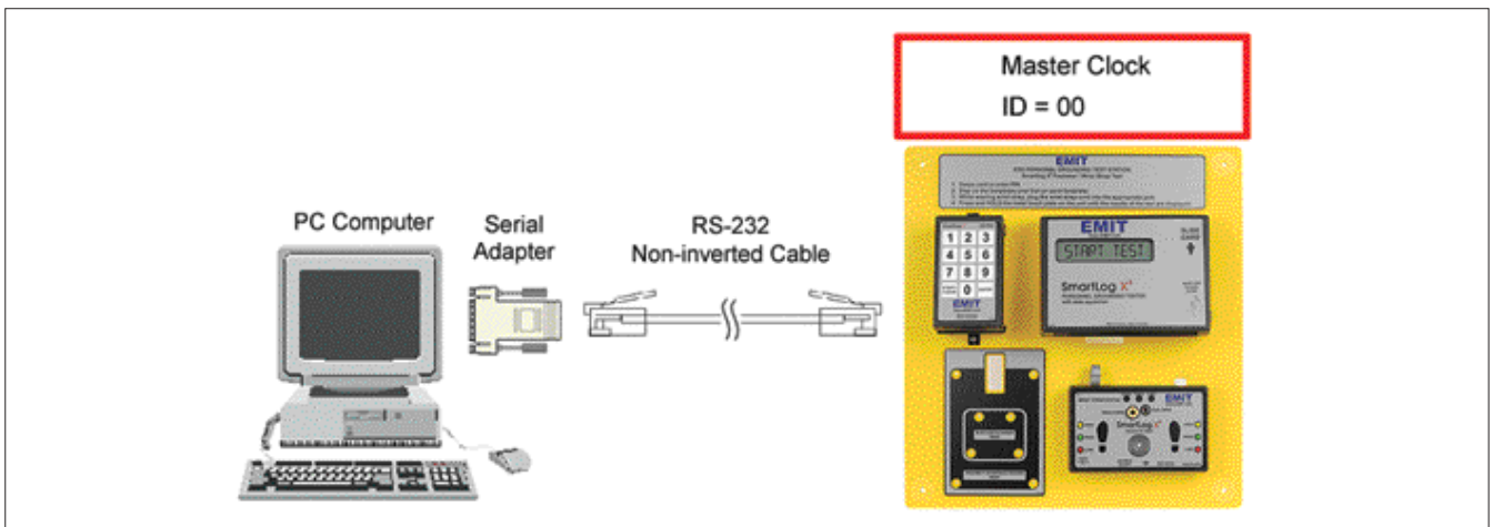
Figure 5. Connecting one SmartLog X 3 ™
