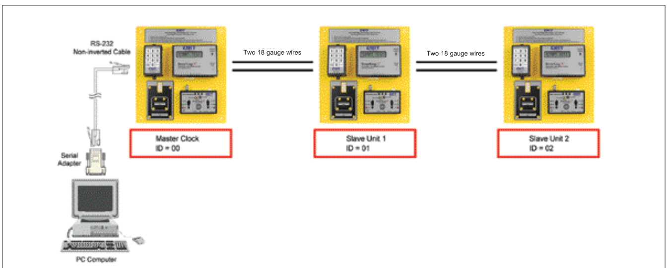
Figure 6. Connecting more than one SmartLog X 3 ™
