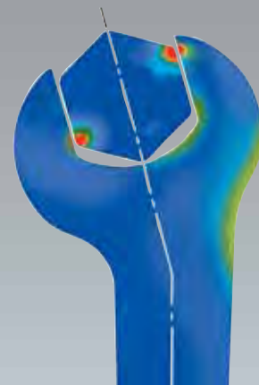
Load zones in spanners by STAHLWILLE
