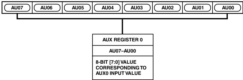
Figure 27. AUX Register 0
