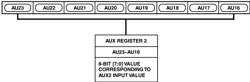
Figure 29. AUX Register 2
