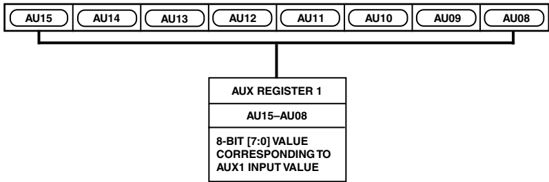
Figure 28. AUX Register 1
