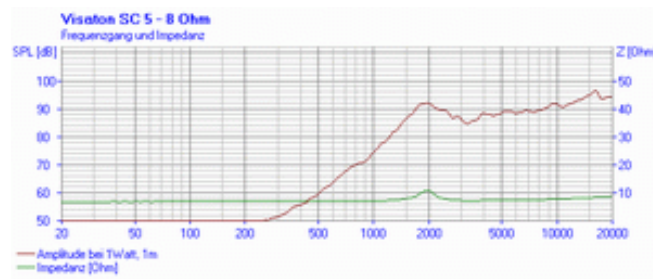
frequency- and impedance response
