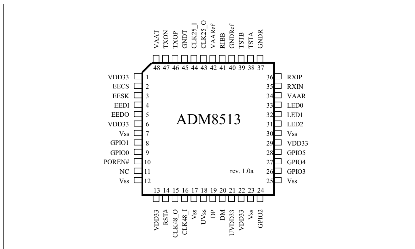
Figure 1 Pin Diagram
