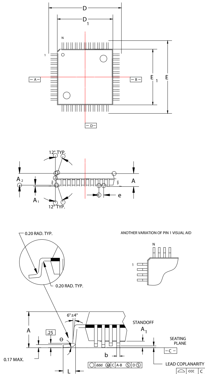
Figure C-1. Stellaris LM3S1W16 64-Pin LQFP Package
