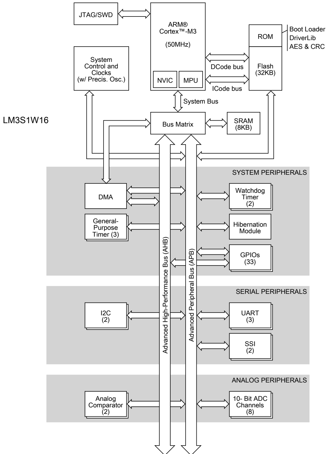
Figure 1-1. Stellaris LM3S1W16 Microcontroller High-Level Block Diagram
