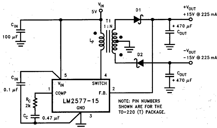
FIGURE 20. Flyback Regulator Easily Provides Dual Outputs
