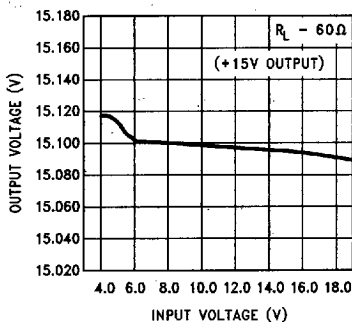
FIGURE 21. Line Regulation (Typical) of Flyback Regulator of Figure 20, +15V Output
