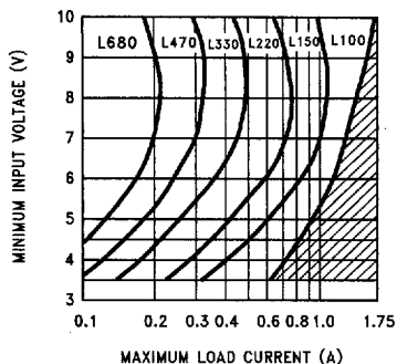
FIGURE 7a. LM2577-12 Inductor Selection Guide
