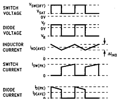
FIGURE 5. Step-Up Regulator Waveforms
