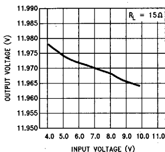
FIGURE 12. Line Regulation (Typical) of Step-Up Regulator of Figure 11
