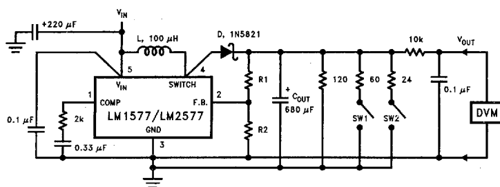
FIGURE 3. Circuit Used to Specify System Parameters for ADJ Versions
