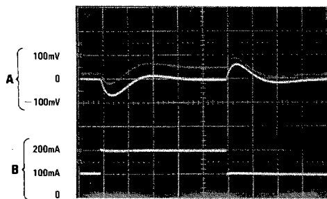
FIGURE 23. Load Transient Response of Flyback Regulator of Figure 20, +15V Output
