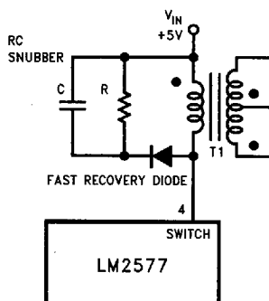
FIGURE 19. Snubber Circuit
