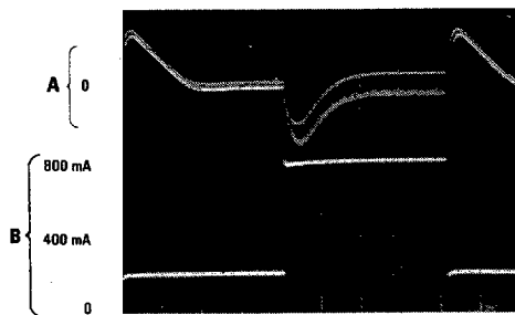
FIGURE 13. Load Transient Response of Step-Up Regulator of Figure 11
