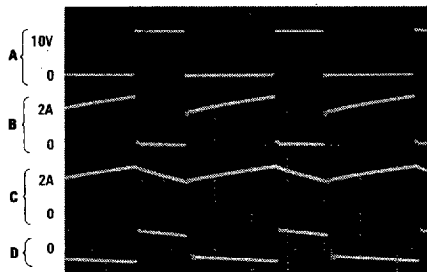
FIGURE 14. Switching Waveforms of Step-Up Regulator of Figure 11
