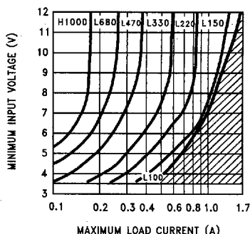
FIGURE 7b. LM2577-15 Inductor Selection Guide
