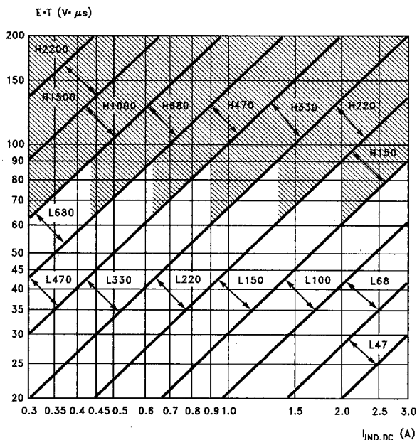
FIGURE 7c. LM1577-ADJ/LM2577-ADJ Inductor Selection Graph
