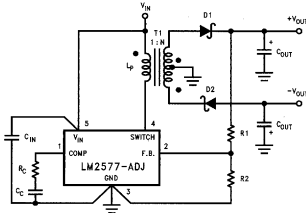
FIGURE 15. LM1577-ADJ/LM2577-ADJ Flyback Regulator with \pm Outputs
