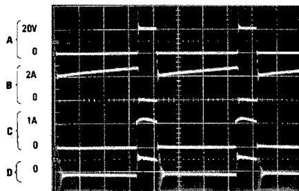
FIGURE 25. Switching Waveforms of Flyback Regulator of Figure 20, Each Output Loaded with 60\Omega
