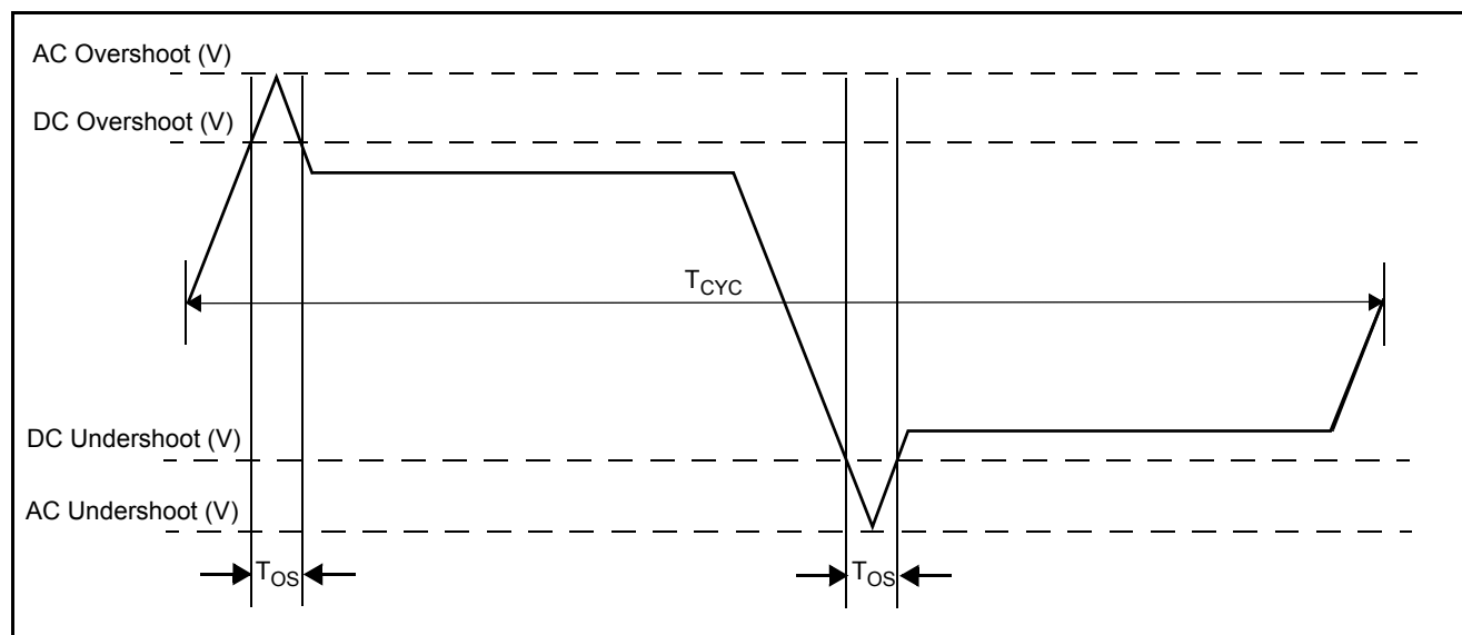
Figure 4. Overshoot Waveform
