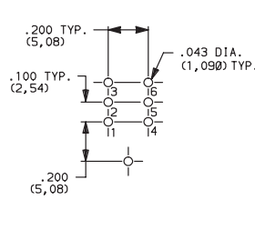
T201MH9AVBE Vertical Actuation DPDT
