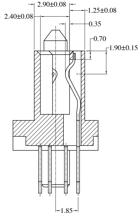
SECTION B-B
