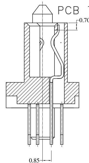
SECTION E-E
