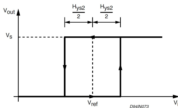
Figure 6. Input comparator threshold
