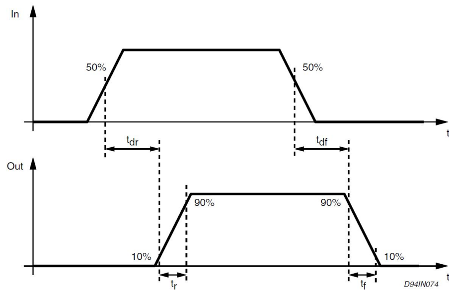
Figure 3. Switching waveforms
