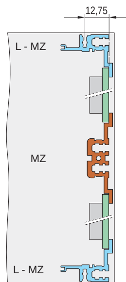
Connector fitting with Z
