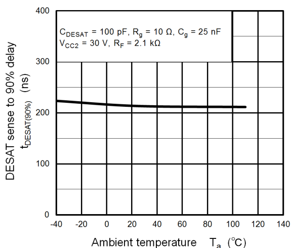
t_{DESAT(90\%)} - T_a
