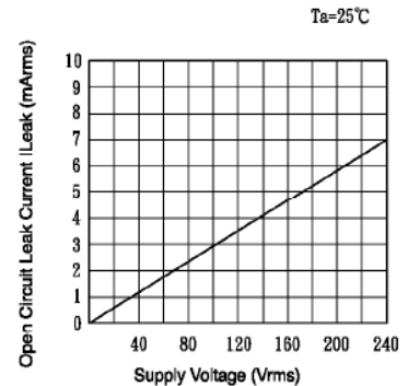
Fig.3 Open Circuit Leak Current vs. Supply Voltage T_a=25^\circ\text{C}
