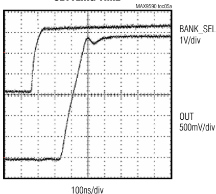
SETTLING TIME
