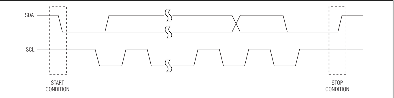
Figure 3. START/STOP Conditions
