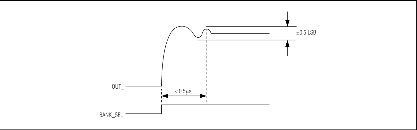
Timing Diagram
