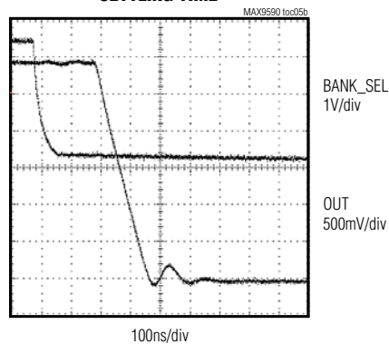
SETTLING TIME
