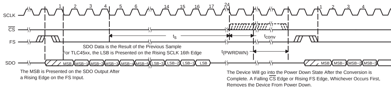
Figure 17. DSP Cycle Timing Using FS Only (or Using Both \overline{\text{CS}} and FS for the TLC4541)
