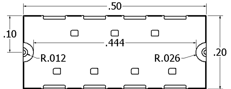
Bottom View
