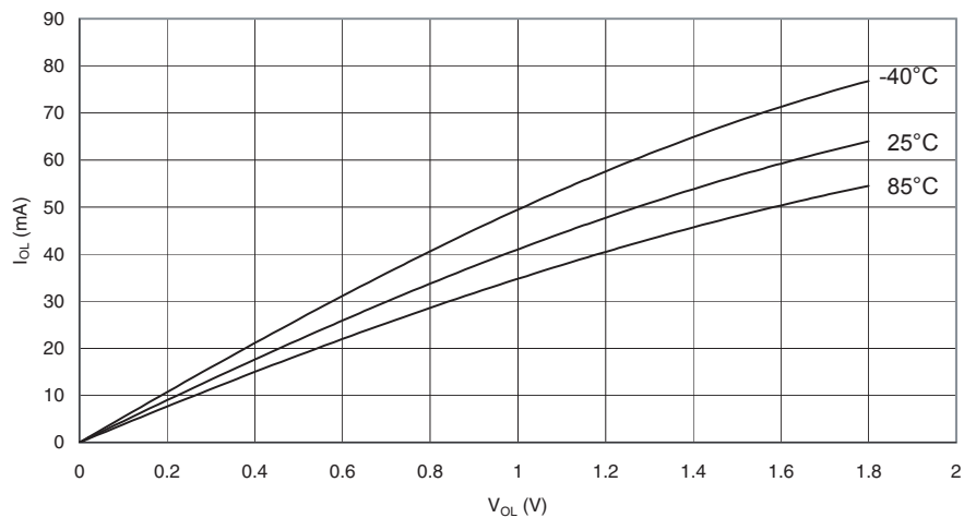
Figure 29-30. I/O Pin Sink Current vs. Output Voltage, Port B ( V_{CC} = 5V )
