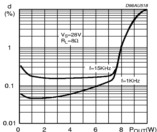
Figure 4: Distortion vs Output Power
