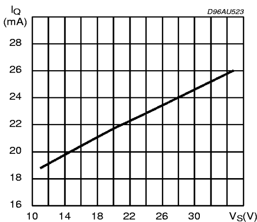
Figure 9: Quiescent Current vs Supply Voltage
