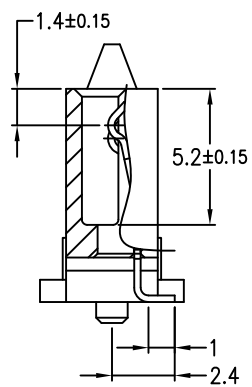
SECT.X-X
