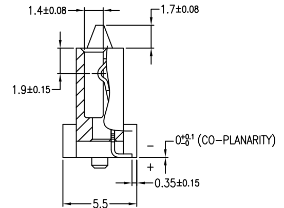
SECT.Y-Y
