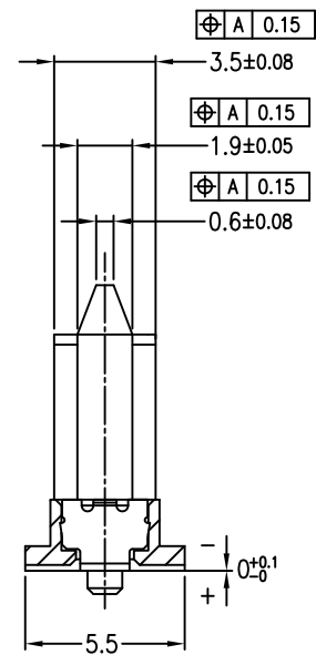
SECT.Z-Z
