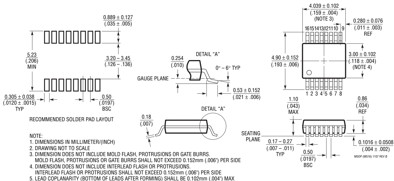
MS Package 16-Lead Plastic MSOP (Reference LTC DWG # 05-08-1669 Rev 0)
